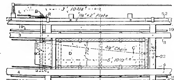
Fig. 322. Part Plan of Door. SLIDE DOOR AND SIDE TRUSSING OF CANADA GONDOLA CAR.
